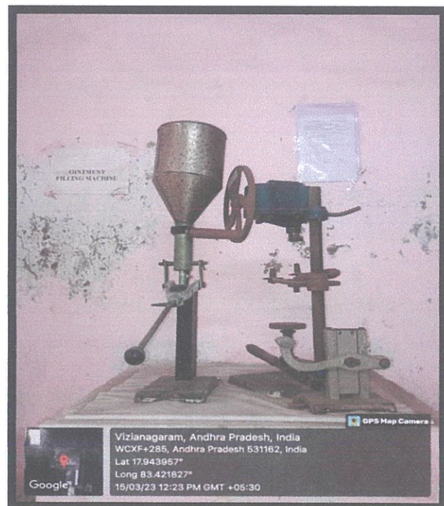
Ointment filling Machine
